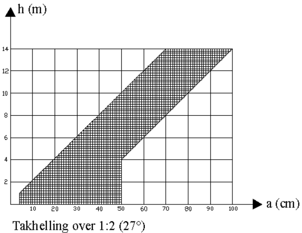
Figur 5c Takhelling over 1:2 (27°)
